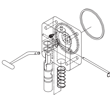
Figure M Disassemble Dispensing Valve
